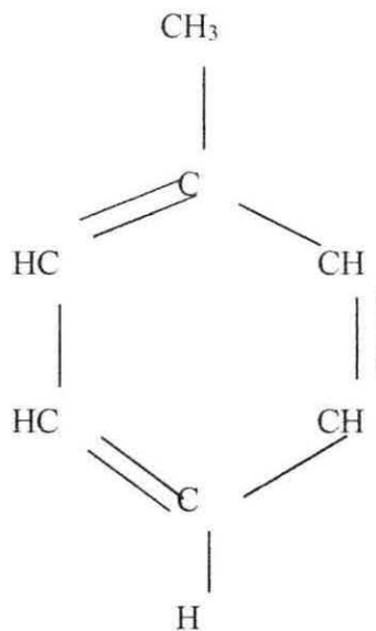
Tolueno
